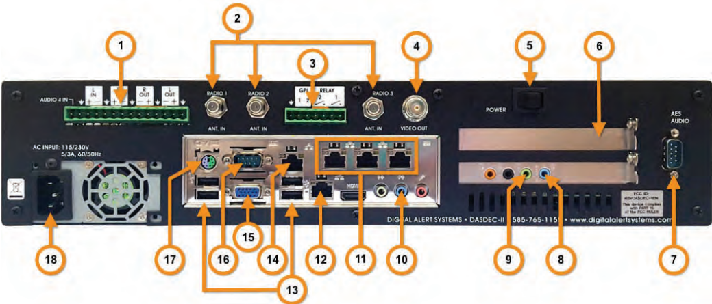
Back Panel
