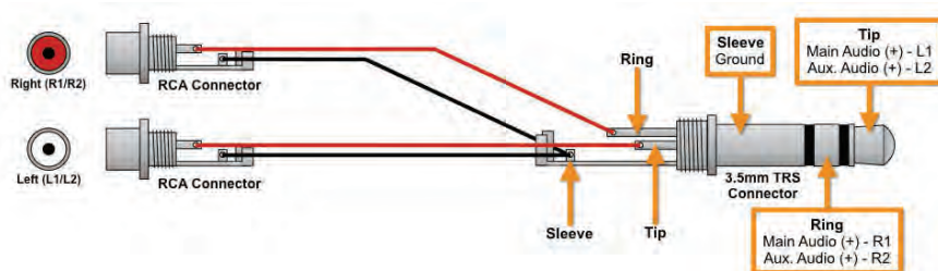
EAS Audio Connectors
